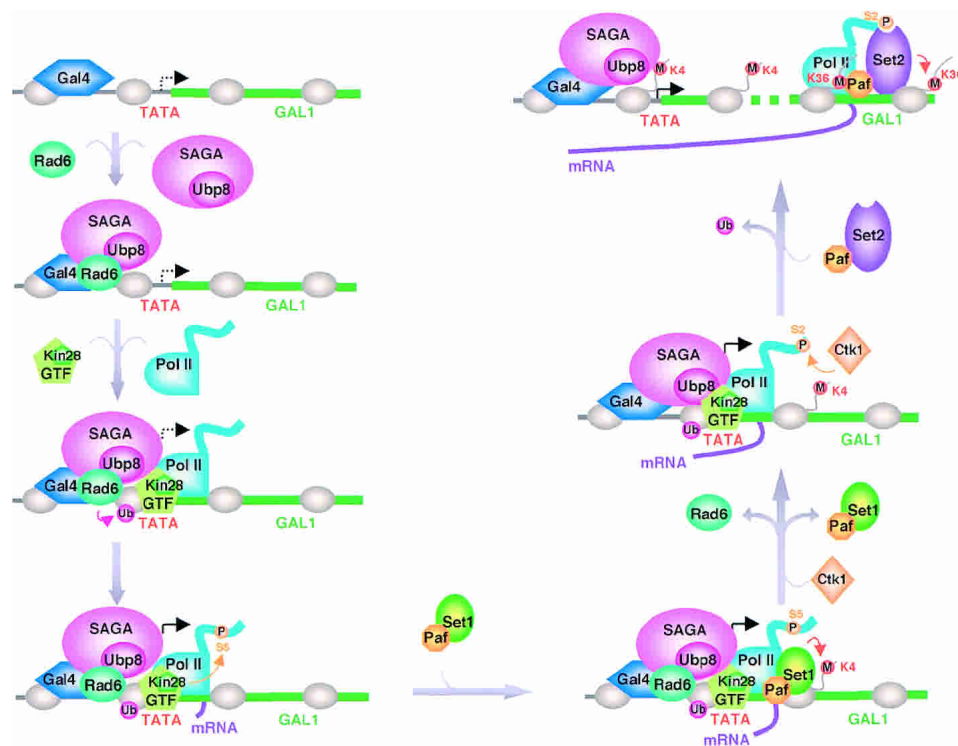
Figure 2. A proposed model depicting the molecular events during transcription of GAL1 gene. Binding of the transcription factor Gal4 to the GAL1 promoter directly or indirectly recruits Rad6 and the SAGA complex. SAGA complex recruits RNAPII and the general transcription factors. Phosphorylation of the CTD on Ser 5 by Kin28 subunit of the TFIIF triggers initiation and elongation of transcription concomitant with the recruitment of the Set1 complex through the Paf1 elongation complex. Set1 complex methylates H3-K4 of the nucleosomes in the promoter and 5' region of the coding region during initiation and early phase of transcriptional elongation. Phosphorylation of the CTD on Ser 2 by Ctk1 may trigger release of Rad6 and Set1 complex from the elongating RNAPII. Ser 2-phosphorylated CTD serves as a docking site for the recruitment of the Set2/Paf1 complex that travels with the elongating RNAPII resulting in H3-K36 methylation in the coding region. Phosphorylation of Ser 2 may also serve as a signal for deubiquitination of H2B. It is important to note that the exact time for some of the events, such as release of Rad6 from the promoter, deubiquitination of H2B and recruitment of Set2, is not known.
