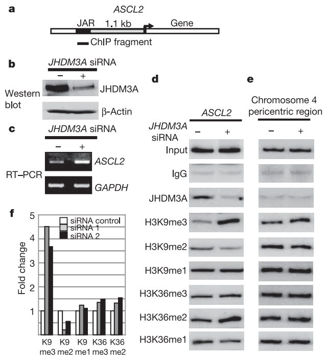
Figure 4 | JHDM3A regulates H3K9/H3K36 methylation at a euchromatic target gene. a, A diagram of the human ASCL2 gene structure. “JAR” represents the “JHDM3A-associated region”. b, JHDM3A protein levels were efficiently reduced by treatment of cells with JHDM3A siRNA. c, siRNA-mediated knockdown of JHDM3A results in increased expression of the ASCL2 gene. d, e, Untreated (–) and JHDM3A -siRNA-treated (+) cells were used in ChIP assays to analyse histone modifications at the ASCL2 gene and the chromosome 4 pericentric region. Reduced levels of JHDM3A caused reduced occupancy of JHDM3A at the ASCL2 gene and increased levels of H3K9me3 and H3K36me2, as assessed by radioactive PCR. JHDM3A was not specifically enriched at the chromosome 4 pericentric regions, and had no effect on the H3K9/H3K36 methylation profiles at this location. f, Quantitative real-time PCR analysis of histone modification levels at the ASCL2 JAR after treatment with two independent siRNAs (see Methods) revealed a increase in H3K9me3 levels and subtle changes in lower H3K9 and H3K36 modifications.
